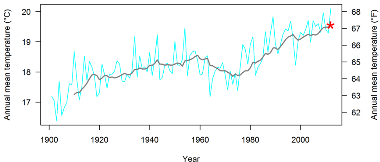
Figure 1. Time series used to characterize the historical range of variability and most recent percentile for annual mean temperature at Saguaro National Park (including areas within 30-km [18.6-mi] of the park’s boundary). The blue line shows temperature for each year, the gray line shows temperature averaged over progressive 10-year intervals (10-year moving windows), and the red asterisk shows the average temperature of the most recent 10-year moving window (2003–2012). The most recent percentile is calculated as the percentage of values on the gray line that fall below the red asterisk (see results of most recent percentiles for all temperature and precipitation variables in Figure 2).
