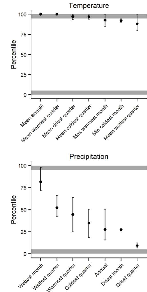
Figure 2. Recent temperature and precipitation percentiles at Saguaro National Park (including areas within 30-km [18.6-mi] of the park’s boundary). Black dots indicate average recent percentiles across the 10, 20, and 30-year intervals (moving windows). Variables are considered “extreme” if the mean percentiles are <5 th percentile or >95 th percentile (i.e., the gray zones, where recent climate is pushing the limits of all observed climates since the year 1901). Black bars indicate the range of recent percentiles across 10, 20, and 30-year moving windows (larger bars indicate higher sensitivity to moving window size).
